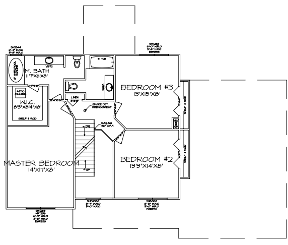
SECOND FLOOR PLAN A-3 SCALE: 1/4\"/>
