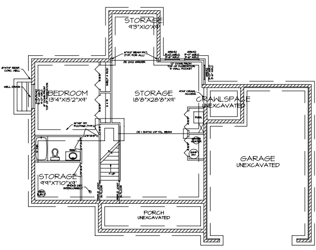
FOUNDATION PLAN A-2 SCALE: 1/4\"/>
