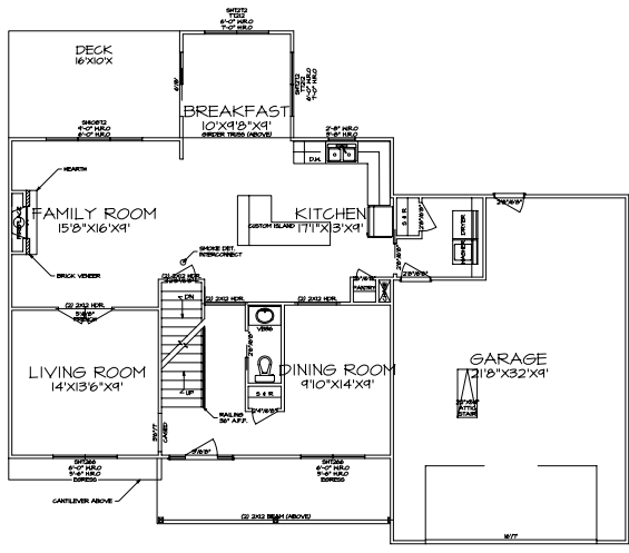
FIRST FLOOR PLAN A-3 SCALE: 1/4\"/>
